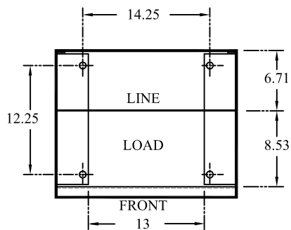
MOUNTING PLAN
